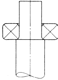
Figure 42. Convention for rolling bearing
